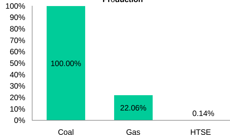
Comparison of Relative CO 2 Emitted for Ammonia Production
