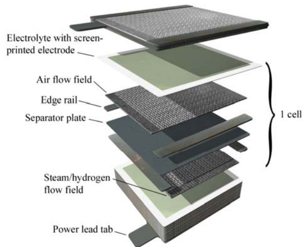
Externally manifolded planar stack, electrolyte-supported cells (Ceramatec)
