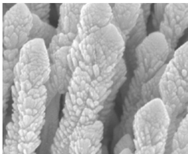
“Whiskerettes” of Pt grow off sides of organic crystalline whisker core
