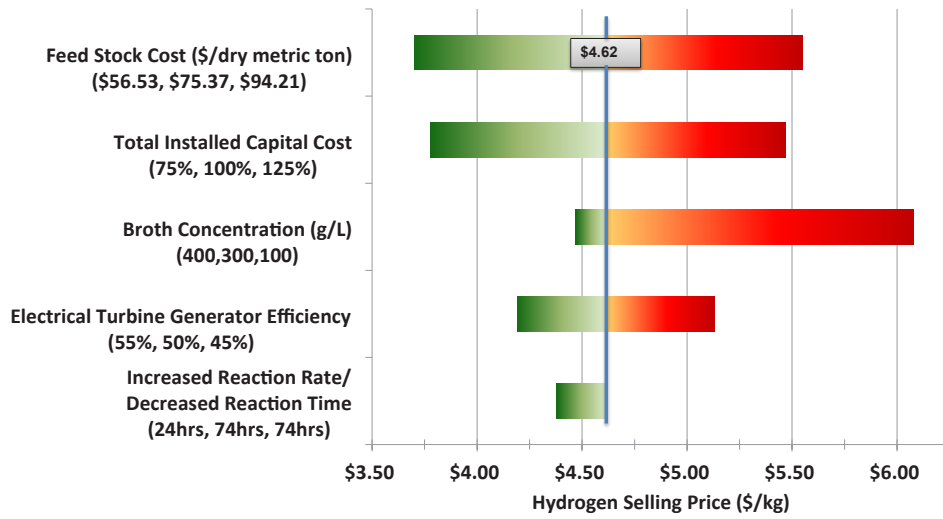
FIGURE 4. Tornado chart for fermentation future case sensitivity study
