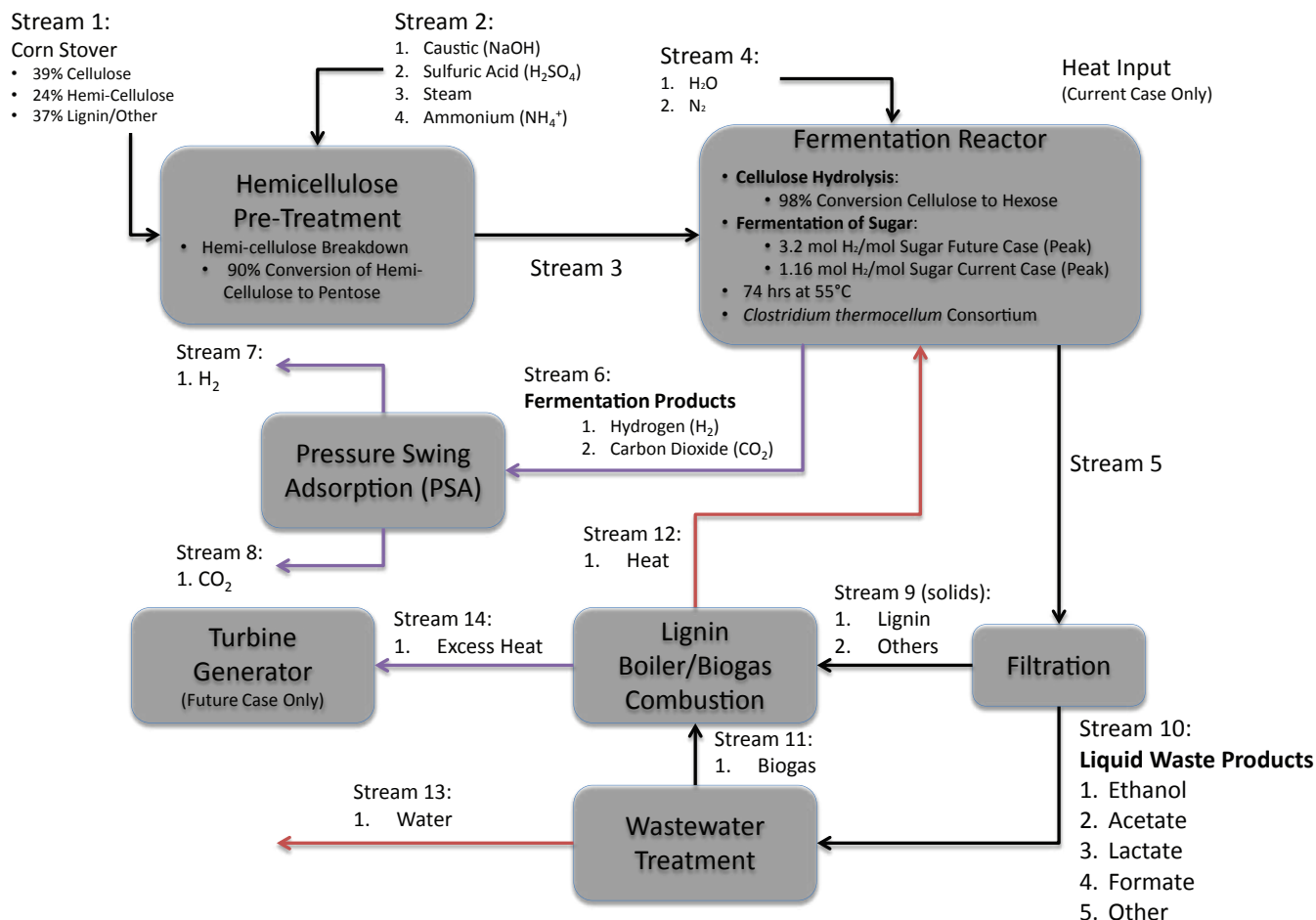
FIGURE 1. Dark fermentation process flow diagram
