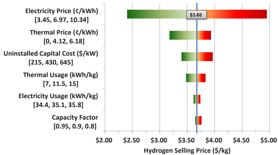
FIGURE 3. Tornado chart for SOEC future case sensitivity study
