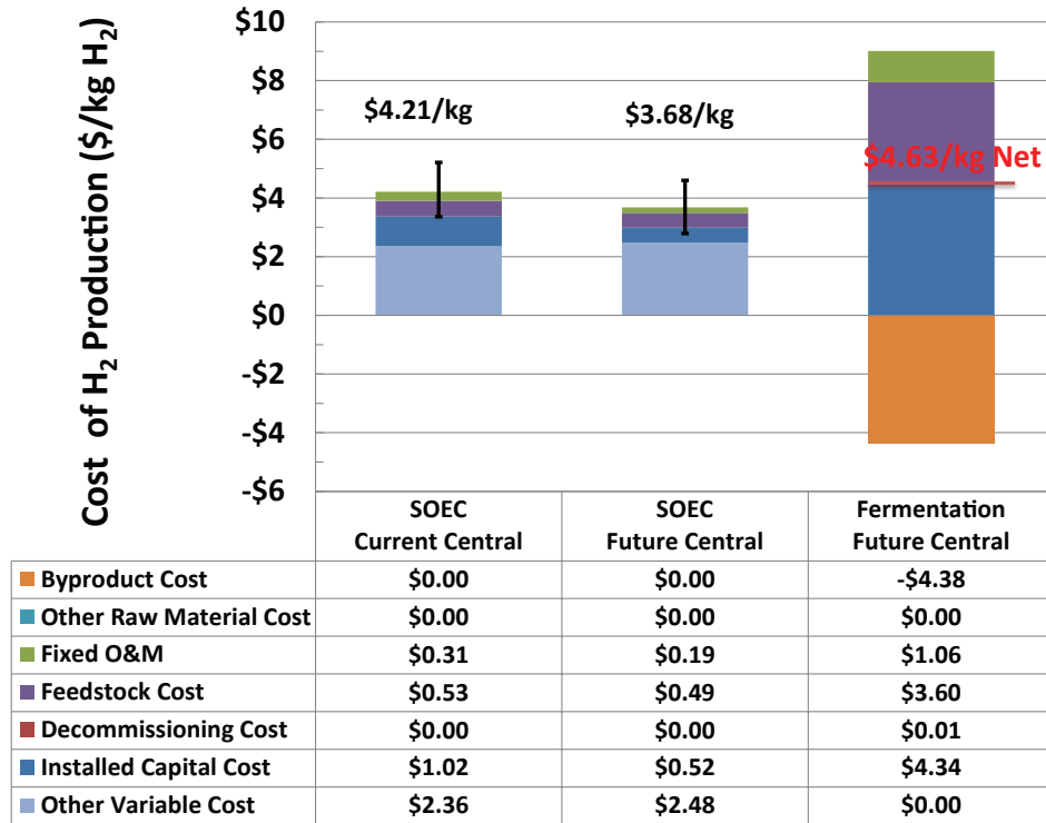
FIGURE 2. Cost breakdown of analyzed systems
