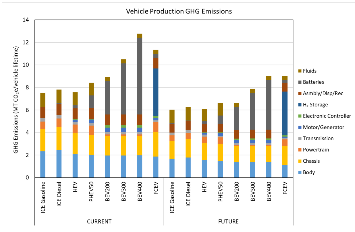
Figure 4. Total Vehicle Manufacturing Cycle GHG Emissions for Current (2020) and Future (2050) Vehicle Powertrain Technologies for Small SUVs
