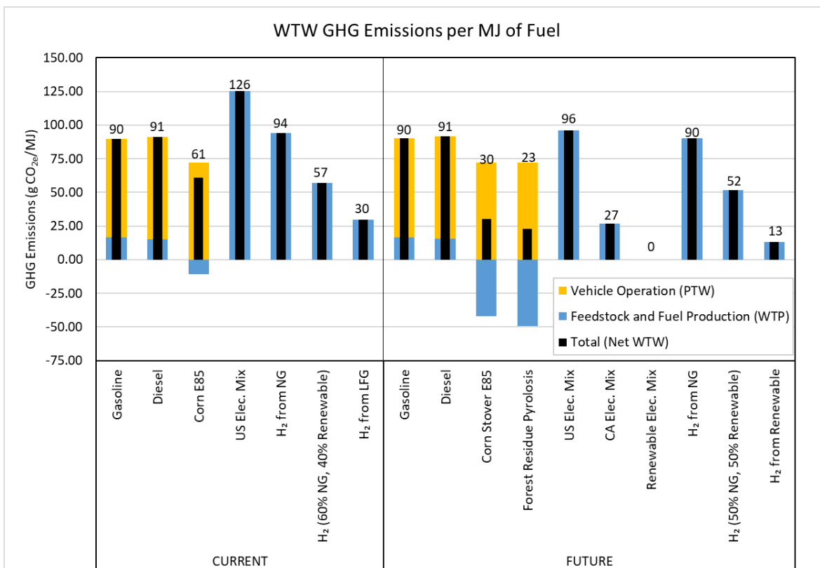
Figure 3. WTW GHG Emissions for Current (2020) and Future (2050) Fuel Technology Pathways
