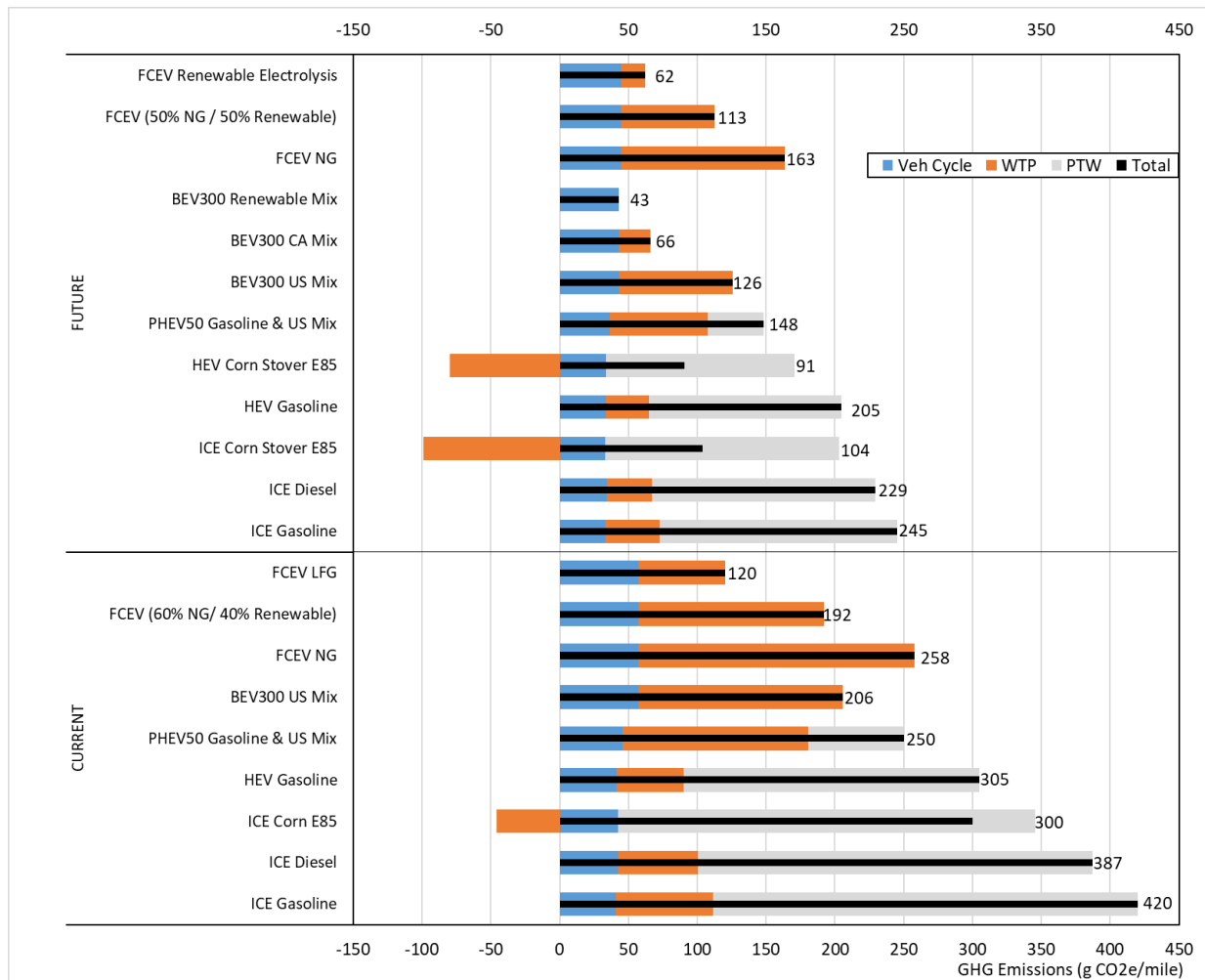
Figure 2. Life Cycle GHG Emissions (g CO 2e /mi) for Selected Current (2020) and Future (2050) Fuels and Vehicle Technologies for Small SUVs
