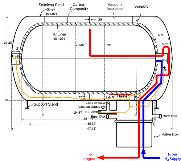
Fig. 1. Design schematic of the LLNL cryo-tank.
