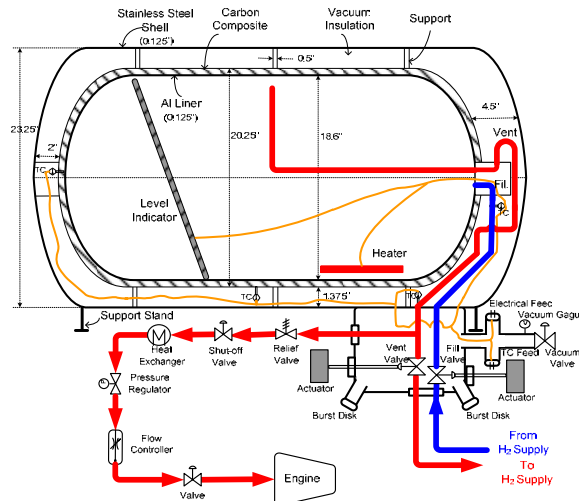
Fig. 4. Modified cryo-tank.
