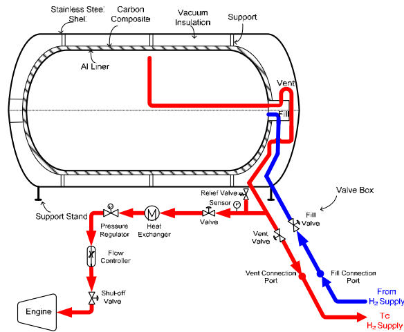
Fig. 2. Design schematic of the ex-vessel components in the LLNL cryo-tank.
