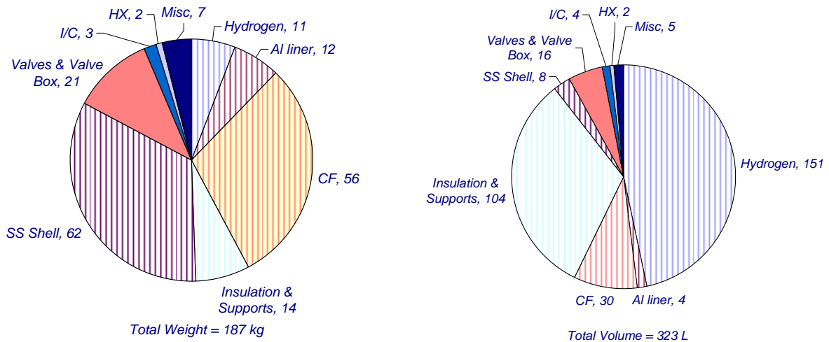
Fig. 3. Weight and volume breakdown by sub-component in the LLNL cryo-tank.
