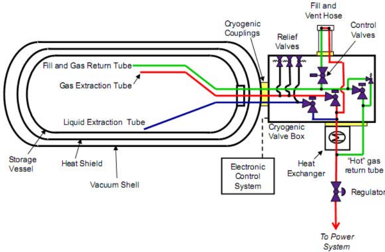
Sketch of Key LH 2 System Components
