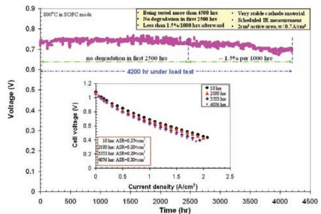
FIGURE 3. 4,200 Hour Long-Term Test (The cell, constructed from a MSRI standard anode tape and deposited with LSCM+SDC-based cathode, was operated in the SOFC mode with a constant load at 800°C. Hydrogen was the fuel and air was the oxidant.)
