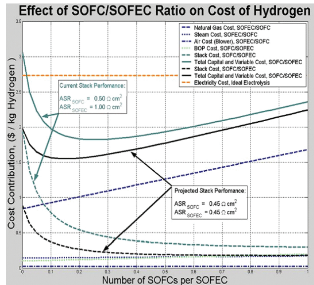
FIGURE 5. Preliminary Cost Analysis Result for Hydrogen Production Based on Hybrid SOFC-SOFEC Technology
