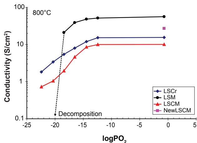
FIGURE 1. Electrical Conductivity of LSCr, LSM and LSCM as a Function of Oxygen Activity at 800^\circ\text{C}
