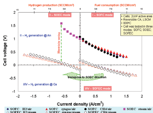
FIGURE 2. Typical Performance Characteristics of a Button-Cell Operated in the Reversible SOFC, SOEC, and SOFEC Modes at 800°C
