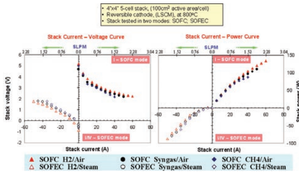
FIGURE 4. Performance of a 5-cell 4"x 4" Stack Operated at 800°C in the SOFC and SOFEC modes. (In the SOFC mode for electricity generation, H 2 , wet syngas with 27% steam, or wet CH 4 with 50% steam was fed to the anode, and air was fed to the cathode. In the SOFEC mode for hydrogen production, H 2 , wet syngas with 27% steam, or wet CH 4 with 50% steam was fed to the anode, and mixture of 70% steam with H 2 as the carry gas was fed to the cathode.)
