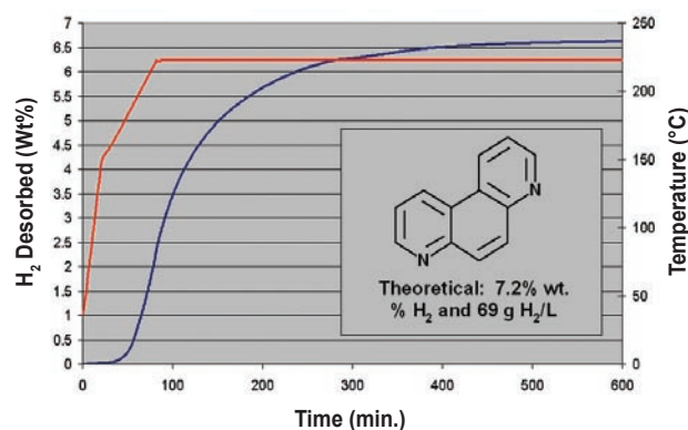
FIGURE 4. Plot of Perhydrophenanthroline Dehydrogenation
