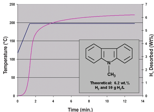
FIGURE 3. Plot of Perhydro-N-methylcarbazole Dehydrogenation
