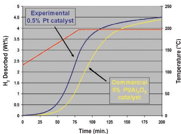
FIGURE 2. Overlay Plot of Dehydrogenation of Perhydro-N-ethylcarbazole with Two Platinum-On-Alumina Catalysts Showing Development of Highly Active Dehydrogenation Catalysts
