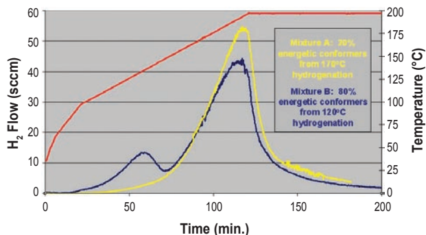
FIGURE 1. Overlay Plot of Dehydrogenation of Two Samples of Perhydro-N-ethylcarbazole Demonstrating Differences between Conformer Mixtures
