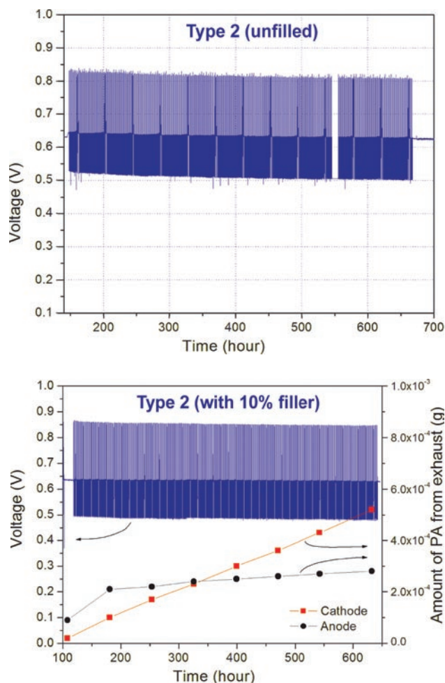
FIGURE 2. Load Cycling Test of Filled and Unfilled Membranes
