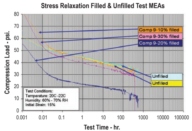
FIGURE 1. Stress Relaxation of Filled and Unfilled Membranes
