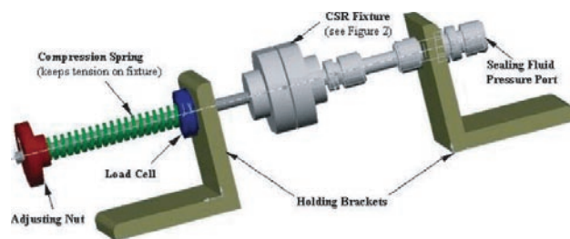
FIGURE 3. Bond Line Strength Test Fixture
