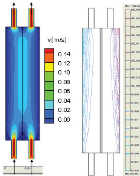
FIGURE 4. CFD results for the Tandem Cells™. The velocity field is shown on the left, and the H + species concentration is shown on the right.
