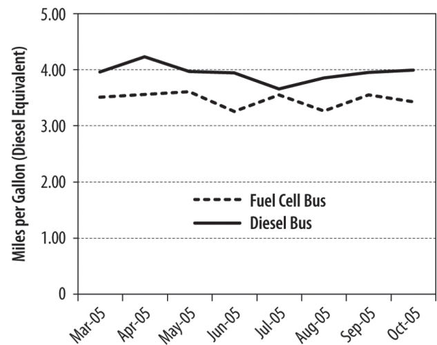
FIGURE 3. Average Fuel Economy by Month
