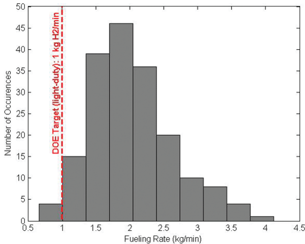
FIGURE 4. Cumulative Fueling Rate Histogram: VTA Station
