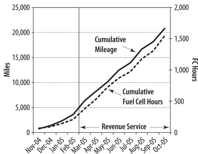
FIGURE 2. Cumulative Miles and Fuel Cell Hours for the three FCBs
