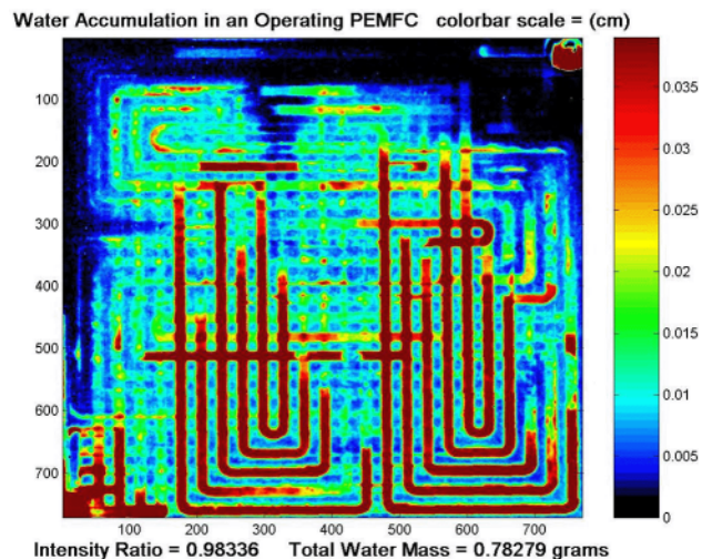
Figure 4. Image of Nearly Uniformly Hydrated Flow Fields and Membrane Assembly
