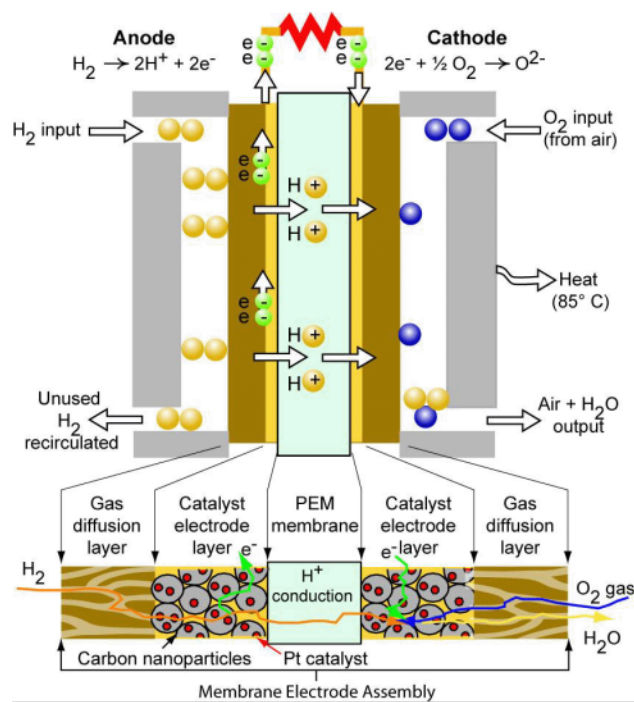
Figure 1. Schematic of a PEM Fuel Cell
