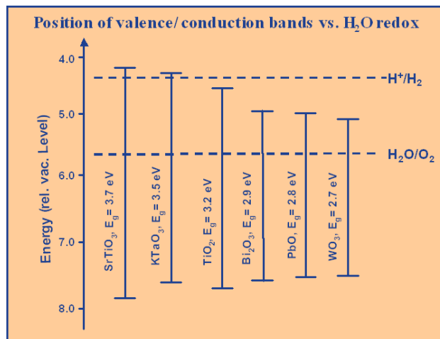
Figure 1. Location of Bandedges of Common Photocatalysts with Respect to Water Redox Potentials
