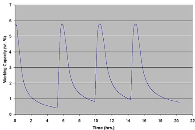
Figure 1. A plot of working hydrogen capacity vs. time for a cycling experiment with N-ethylcarbazole in a batch reactor with a slurry of hydrogenation catalyst and dehydrogenation catalyst. The hydrogenation conditions are 170°C and 1200 psia H 2 , and the dehydrogenation is performed with a temperature ramp from 30 to 200°C over 1.75 hours, holding at 200°C, all under 15 psia H 2 .
