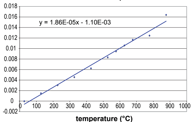
FIGURE 2. Lattice parameters (corrected for instrumental errors) determined from 25–900°C indicate a thermal expansion coefficient of 18.6 \times 10^{-6} .
