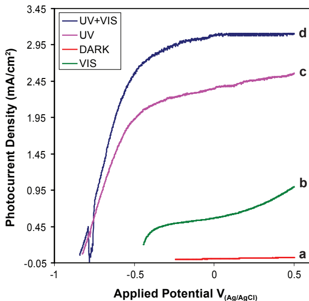
FIGURE 3. Variation of photocurrent density vs. applied potential of the \text{TiO}_2\text{-C}_x nanotubular arrays in (a) dark, and (b) illumination of visible ( 520 \pm 46 nm), (c) UV ( 330 \pm 70 nm) and (d) complete solar spectrum. The efficiency for the above photoelectrochemical cell is calculated as 13.3% using UV light source and 8.5% using visible light source. (Please see Mohapatra et al., Journal of Physical Chemistry: C 111 (2007) 8677-8685 for a detailed discussion on efficiency calculation.)
