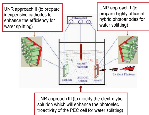
FIGURE 1. A schematic view of the approaches adopted by UNR to develop a highly efficient PEC cell for water splitting. The combination of the three approaches (I + II + III) are expected to give >12% efficiency to generate H_2 from water using sunlight.
