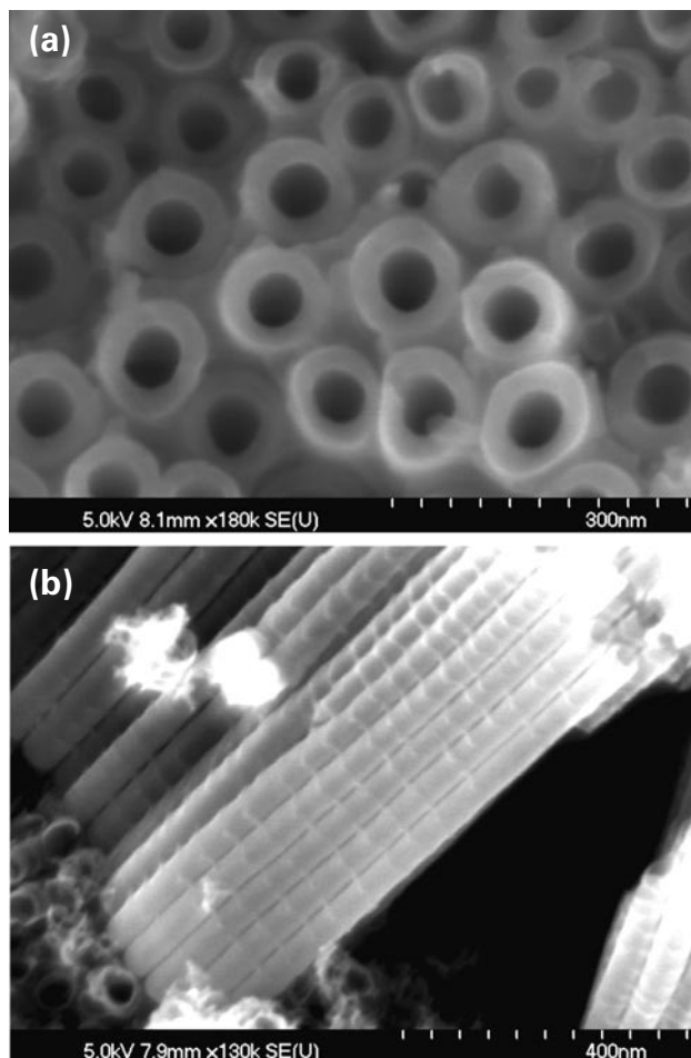
FIGURE 2. Highly Ordered and Compact TiO_2 Nanotube Arrays Prepared by Sono-electrochemical Anodization Method Developed at UNR; (a) top view and (b) side view of the nanotubular array
