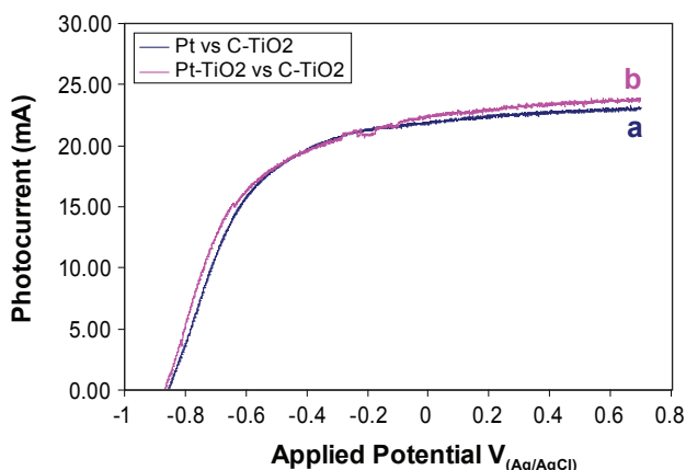
FIGURE 4. Variation of photocurrent obtained from the PEC cell using an 8\text{ cm}^2 photoanode containing \text{TiO}_2\text{-C}_x nanotubular arrays (prepared using the condition earlier mentioned for Figure 2B and annealed under reduce atmosphere) vs. (a) Pt foil and (b) platinum nanoparticles containing titania ( \text{Pt/TiO}_2 ) nanotubular arrays as a cathode.
