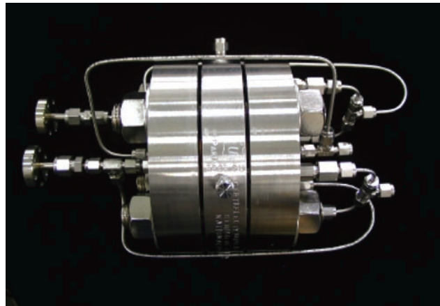
FIGURE 1. A 1.3 pounds/day Hydrogen Separation Unit Designed by NORAM.
