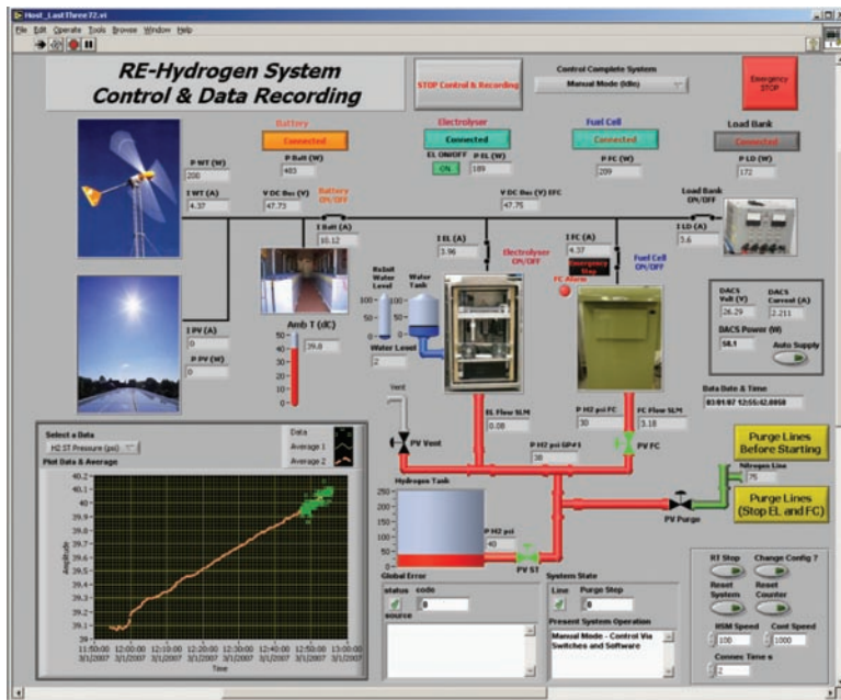
FIGURE 1. Component Testing at the HFCTF
