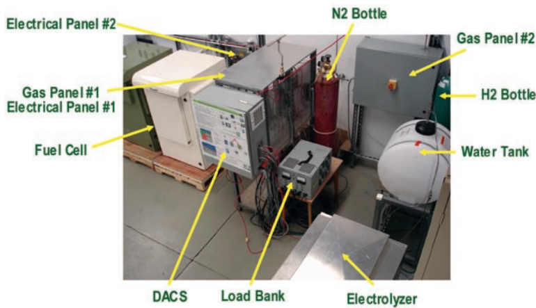
FIGURE 1. Component Testing at the HFCTF
