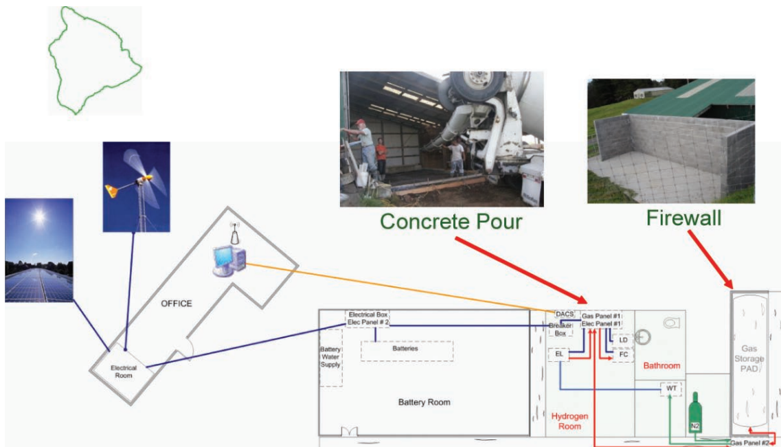
FIGURE 4. Kahua Ranch Infrastructure
