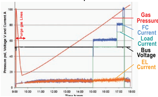
FIGURE 3. Validation of Components and Control System
