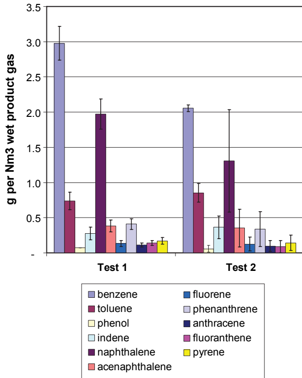
FIGURE 6. Results of Analysis of Tar Species in the Product Gas from the HNEI Bench-Scale Gasifier at an Equivalence Ratio of 0.26, Steam to Biomass Ratio of 0.3, and Gasifier Reactor Temperature of 800°C
