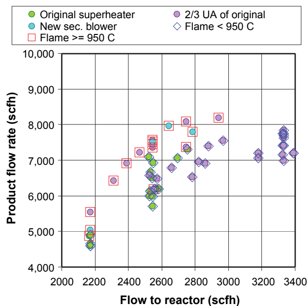
FIGURE 1. Hydrogen Production Rate as a Function of NG Flow to the Reformer
