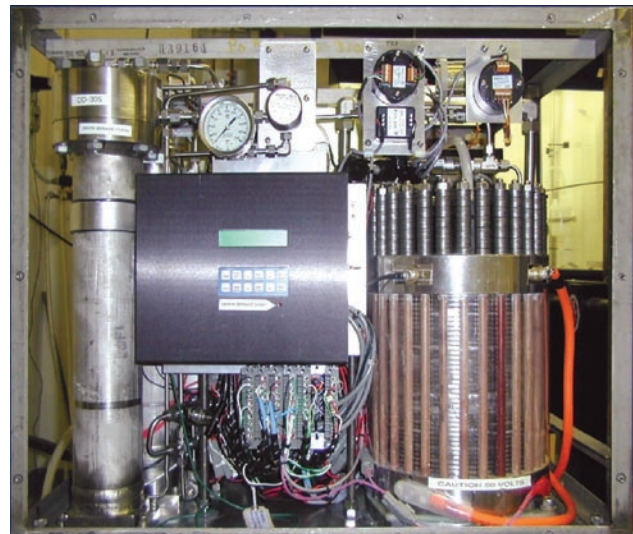
FIGURE 2. EP-1 Electrolyzer Module Delivered to NREL for Field-Testing
