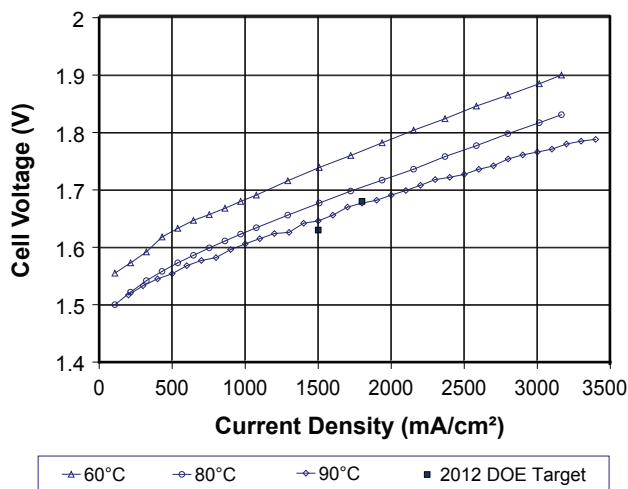
FIGURE 1. Performance of DSM Following 300 Hours of Operation
