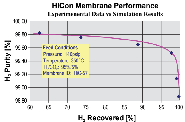
FIGURE 1. Performance of Membrane with Improved Hydrogen Selectivity Targeting Production of >99% Purity as Feed for Polishing Step
