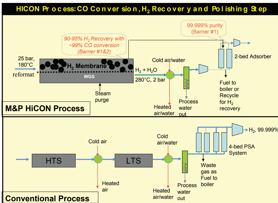
FIGURE 2. Comparison of M&P HiCON Process vs. Conventional Process. Also Shown are the Barriers Overcome by Our Proposed Process.
