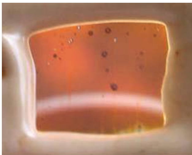
FIGURE 2. Morphology of a-SiC photoelectrodes after the 100-hour durability test. Illumination is from the backside of the samples.
