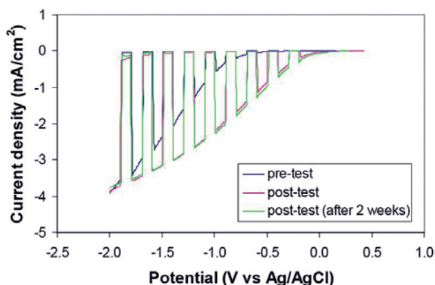
FIGURE 3. IV characteristic measured on an a-SiC photoelectrode before (blue line), right after (pink line) and two weeks after (green line) to the 100-hour durability test.
