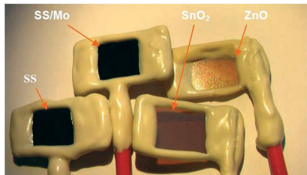
FIGURE 4. Surface morphology of a-SiC photoelectrodes on Pt-coated SS, SS/Mo, ZnO and SnO_2 substrates after 24-hour test.
