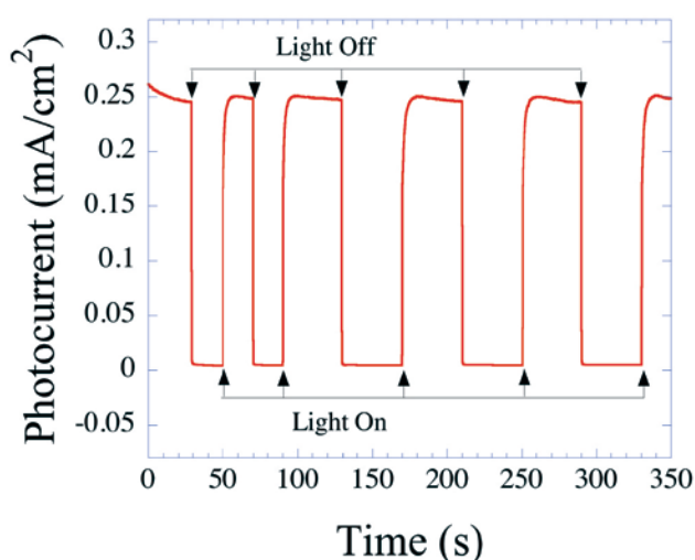
FIGURE 2. Photocurrent from self-biased photochemical diode comprised of an n-type \text{TiO}_2 nanotube array – p-type Cu-Ti-O nanotube array under global AM 1.5 illumination (geometry shown in Figure 1 ). Light is incident upon the oxygen evolving \text{TiO}_2 side of the diode, with the visible portion of the spectrum passing to the Cu-Ti-O side. The n- \text{TiO}_2 side of the diode is kept immersed in a 1M KOH aqueous solution, the p-Cu-Ti-O side is kept in 0.1M \text{Na}_2\text{HPO}_4 with a salt bridge linking the two solutions.
