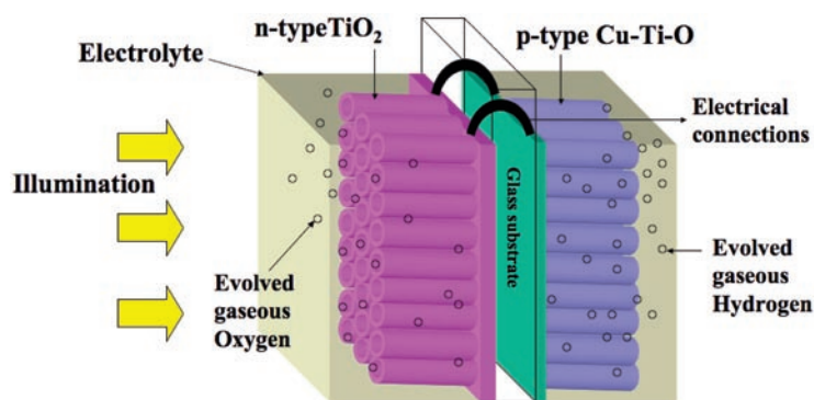
FIGURE 1. Illustration of photoelectrochemical diode for water splitting comprised of n-type \text{TiO}_2 and p-type Cu-Ti-O nanotube array films, with their substrates connected through an ohmic contact. The oxygen evolving \text{TiO}_2 side of the diode absorbs UV light, passing the visible light to the hydrogen evolving Cu-Ti-O side.
