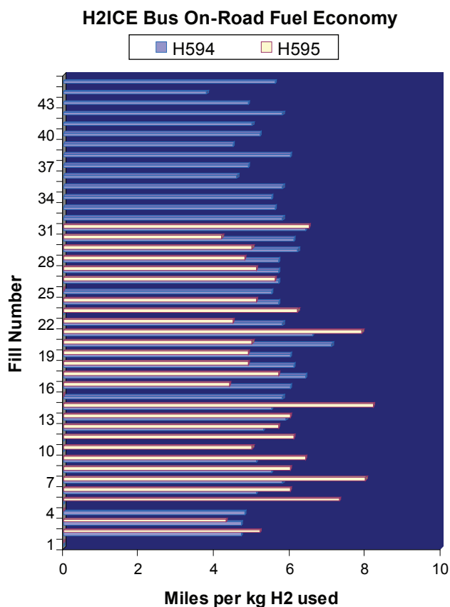
FIGURE 1. H2ICE Bus On-Road Fuel Economy
