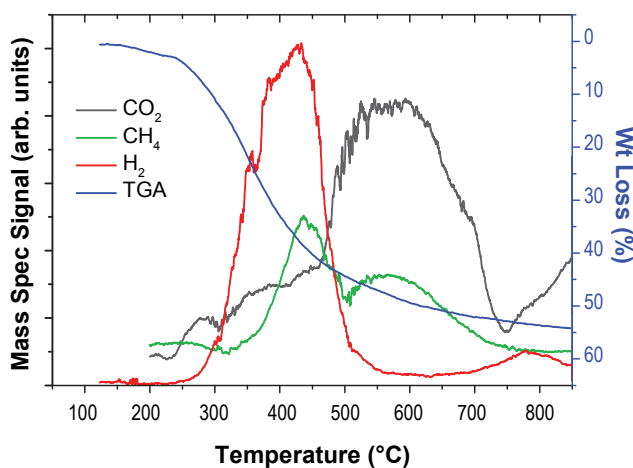
FIGURE 5. Low-Temperature, Catalytic Pyrolysis of Lignin (T ramp rate = 5°C/min, N 2 purge rate = 30 ml/min)
