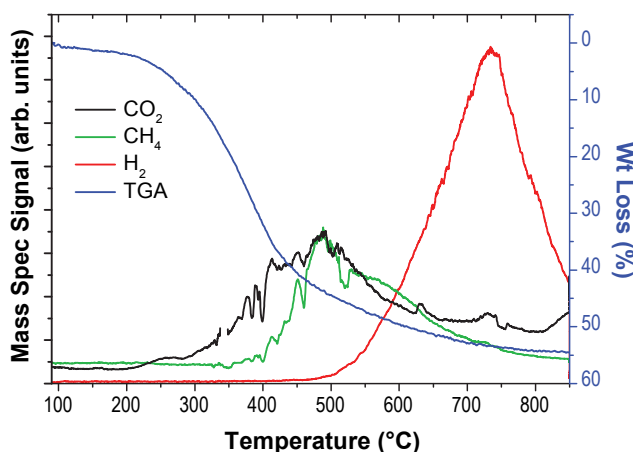
FIGURE 4. Lignin Pyrolysis in the Absence of a Catalyst (T ramp rate = 5°C/min, N 2 purge rate = 30 ml/min)
