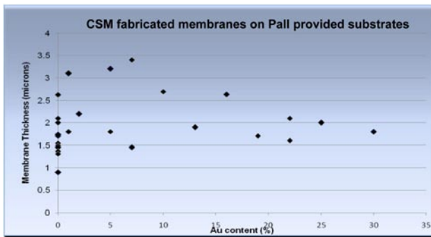
FIGURE 1. Reproducibility of Membrane Synthesis Process to Produce a Narrow Thickness Range
