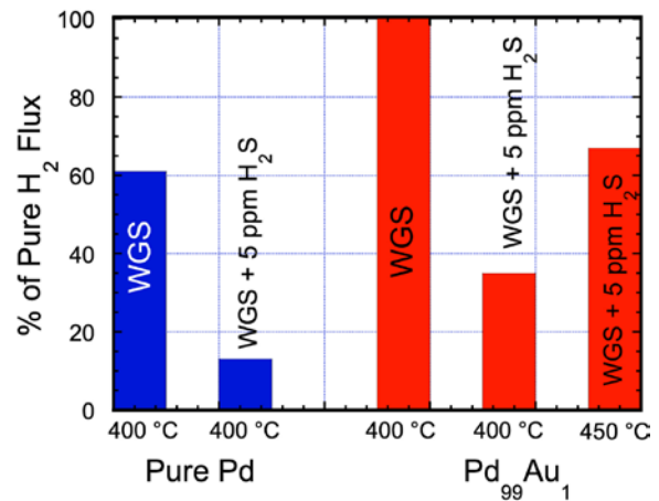
FIGURE 3. Effect of H 2 S on Pd-Alloy Membranes
