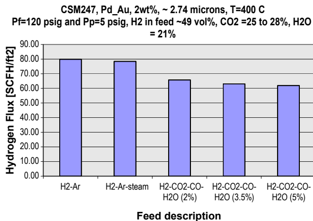
FIGURE 2. Effect of Steam and Carbon Monoxide on Membrane Hydrogen Flux Rate
