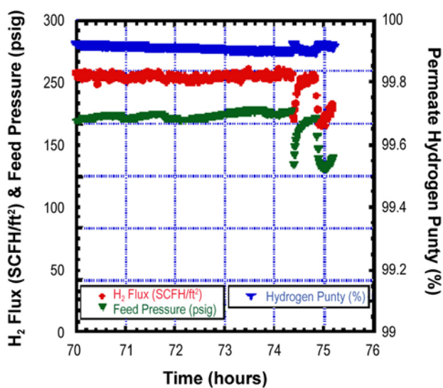
FIGURE 4. Membrane Performance in High Pressure Post-WGS Synthesis Gas Environment
