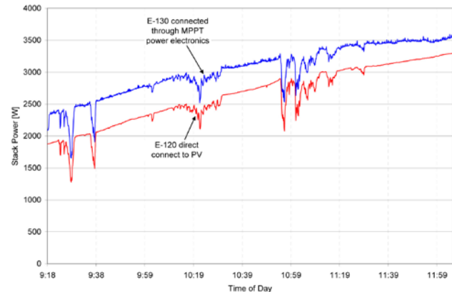
FIGURE 2. Energy Transfer Improvements for MPPT Power Electronics over Direct Connect for 5 kW PV Array to PEM Electrolyzer Systems
