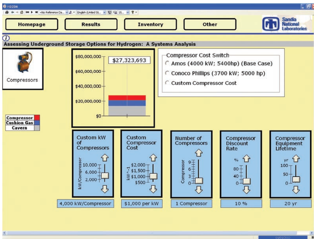
FIGURE 2. Salt Cavern Compressor Cost Module (as of June 2009)
