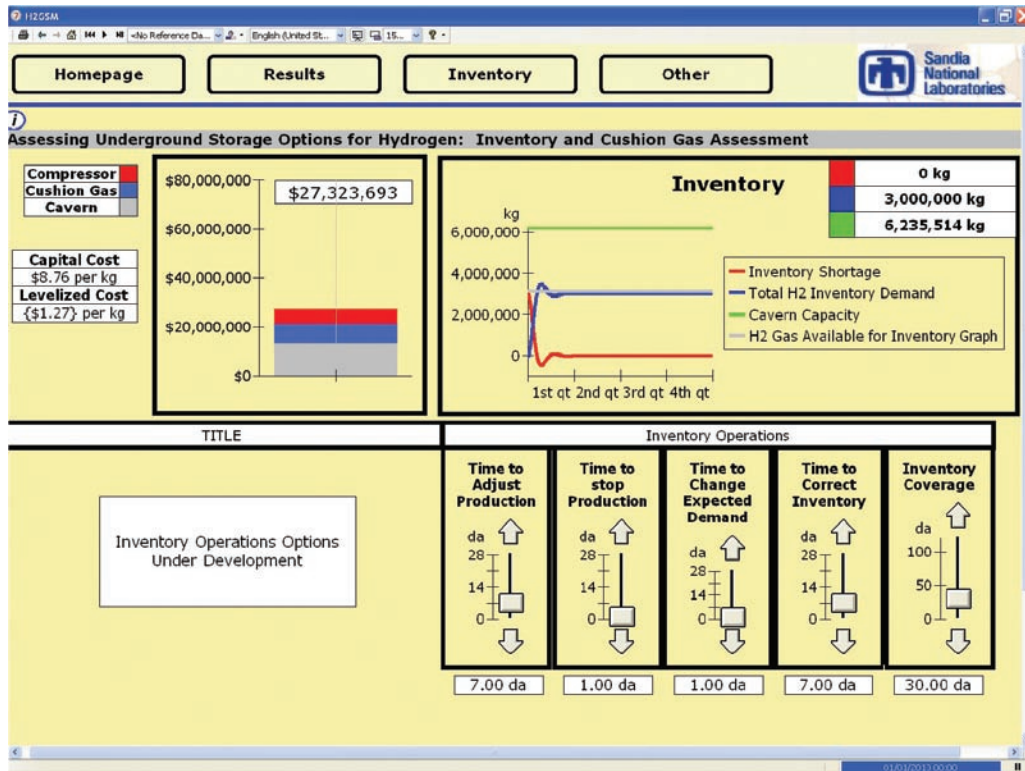
FIGURE 3. Salt Cavern Inventory Model (as of June 2009)
