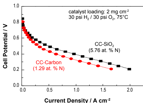
FIGURE 1. Current-voltage plot of PEM fuel cells using CC-SiO 2 and CC-Carbon catalysts at 75°C. The cathode catalyst loading was 2.0 mg cm -2 . The tests were run using H 2 and O 2 with back pressures of 30 psi/30 psi.
