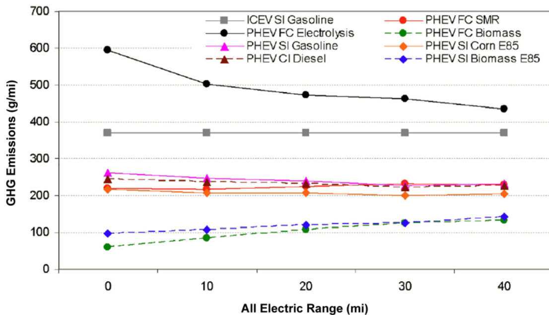
WTW GHG Emissions of PHEV Options Vary Among Fuel Options (US Mix for PHEV Recharge)
