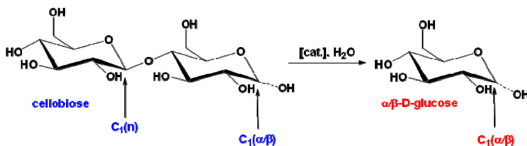
FIGURE 2. Schematic of Cellobiose to Glucose Reaction
