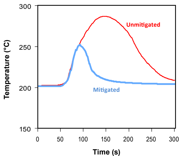
FIGURE 3. A comparison is shown for materials with and without mitigation polymer. It can be observed that the energy released is reduced by nearly 70%, indicating significant progress in mitigation technology development.
