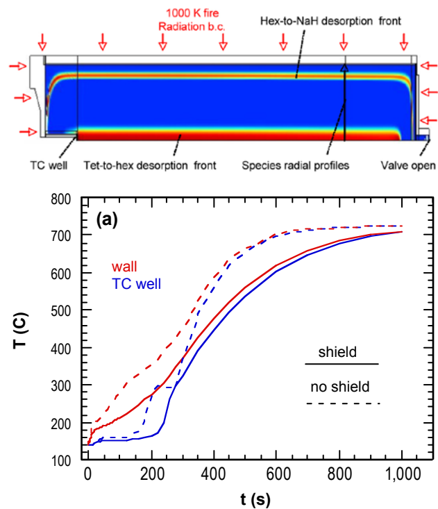
FIGURE 2. Axisymmetric model assembled for analysis of the fire impingement scenario involving a sodium alane containing system. Results indicate that the over-temperature condition can be delayed with the use of simple thermal shielding.
