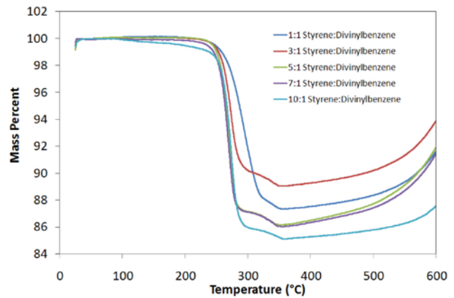
FIGURE 4. TGA comparison of various cross-linking densities indicates little change in decomposition behavior in spite of large structural properties changes.
