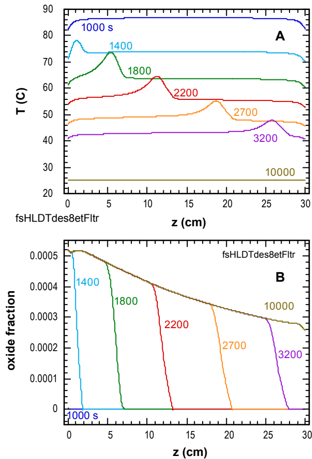
FIGURE 1. Breach-in-tank scenario for a desorbing alane bed. A moderate reaction front proceeds for nearly 1 hour (A) with only a small fraction of the alane oxidized (B).
