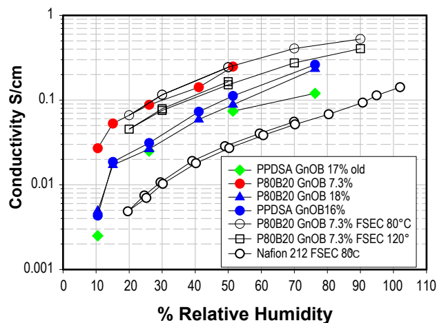
FIGURE 3. Conductivity of nOB-grafted materials, including results from Florida Solar Energy Center. Measurements were at 80°C unless otherwise indicated.
