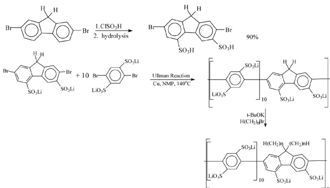
SCHEME 1. Approach to Synthesis of New Random Copolymer, P10F1, and Preparation of Water Insoluble Materials for PEMs
