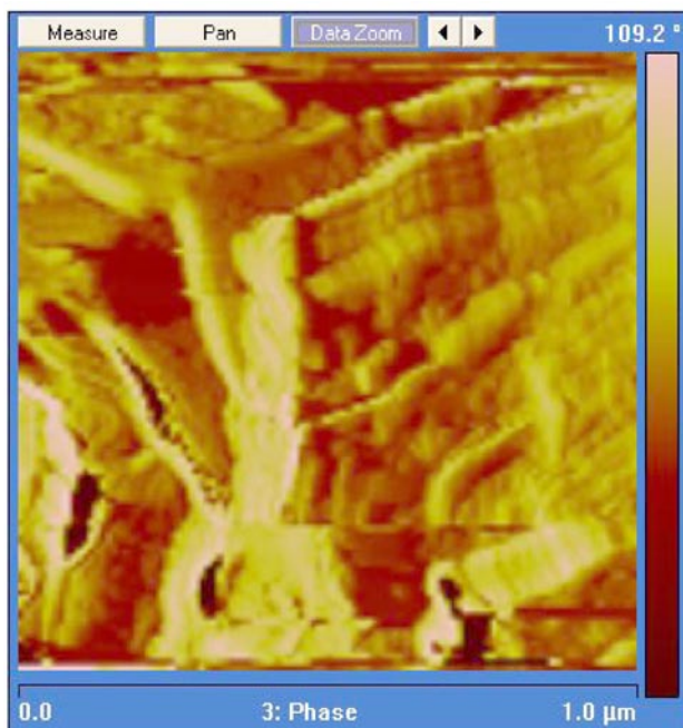
FIGURE 4. AFM Scan of CPPSA-3, Na Salt, after Preliminary Sonication
