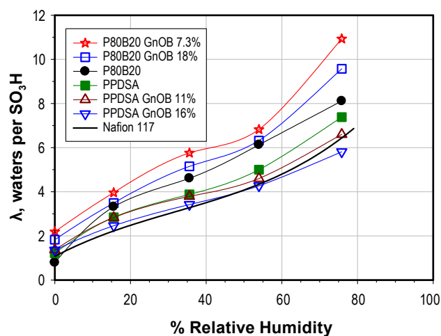
FIGURE 2. Lambda as a function of RH for PPDSA, P80/B20 copolymer and their grafts with nOB compared with Nafion117® [5].
