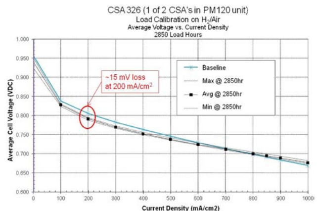
FIGURE 3. Characterization of stack performance (expressed per cell) at BOL (baseline) and following membrane failure in the field. Max/min represents +/- 1 \sigma substack voltages.
