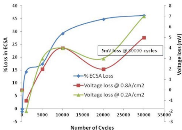
FIGURE 6. Diagnostics Results from PGM Decay AST
