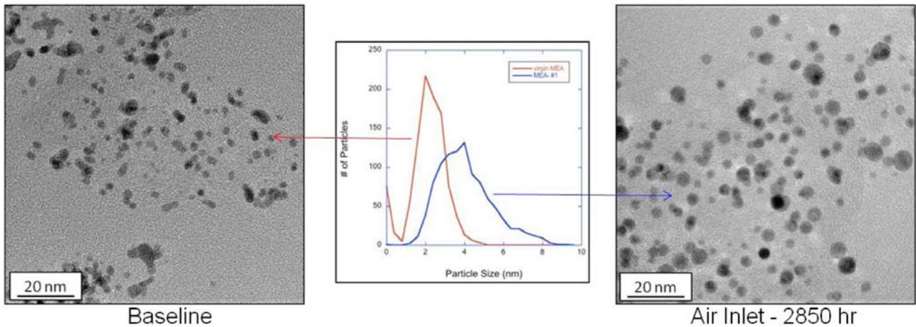
FIGURE 5. TEM Cathode Catalyst Images for Baseline and 2,850 h Catalyst Samples from Air Inlet Region
