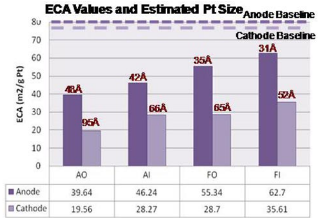
FIGURE 4. ECA data obtained from a 2,850 h cell using cyclic voltammetry. Baseline values are averages from unused samples. Pt particle sizes estimated from XRD are given at the top of the bars (from 2010 DOE Annual Merit Review FC015 – June 8 th 2010).
