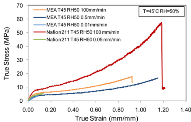
FIGURE 4. Tensile Test Results for MEA and NAFION® 211 membrane at T=45°C and RH=50%
