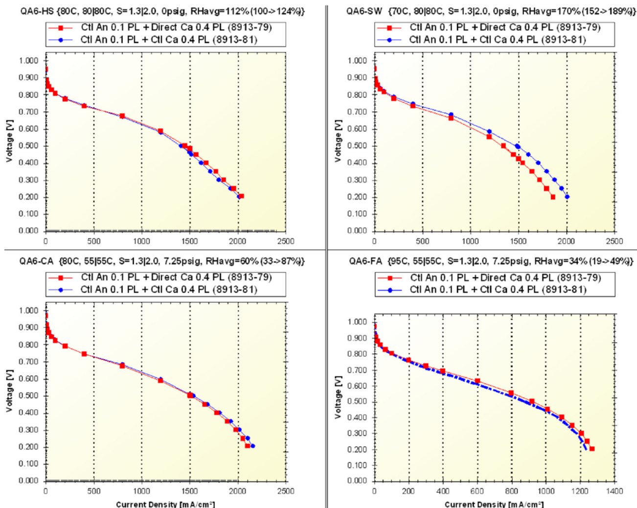
FIGURE 2. Direct-Coated Cathode Performance (PL = platinum loading in mg/cm 2 )
