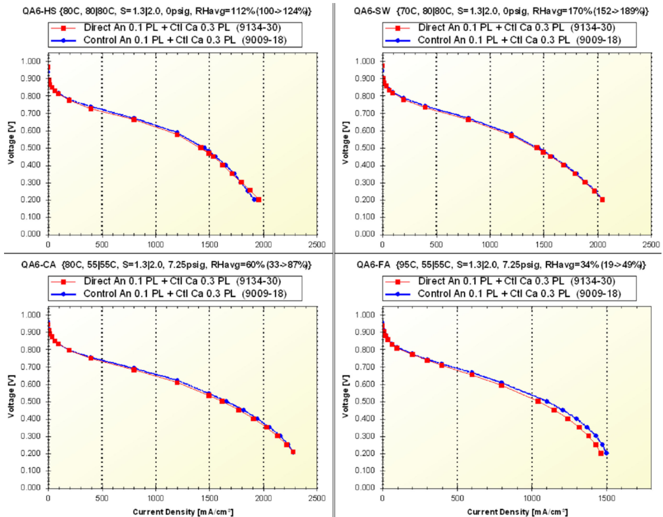
FIGURE 1. Direct-Coated Anode Performance (PL = platinum loading in mg/cm²)
