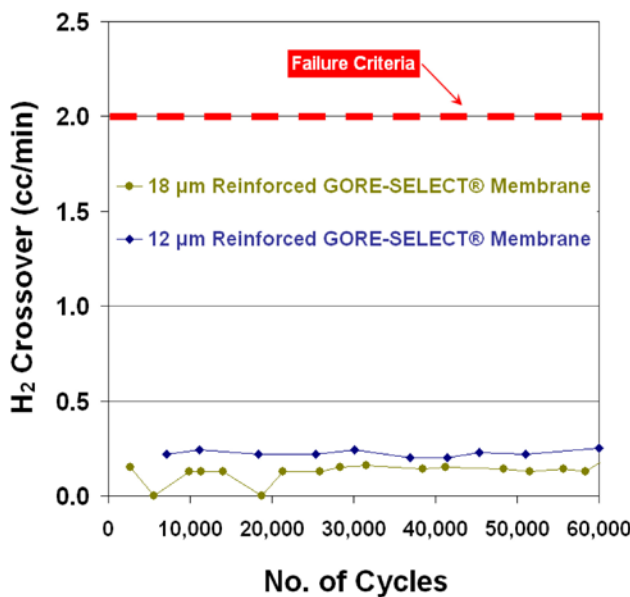
FIGURE 3. Accelerated Mechanical Durability Test Data for 12 μm GORE-SELECT Membrane
