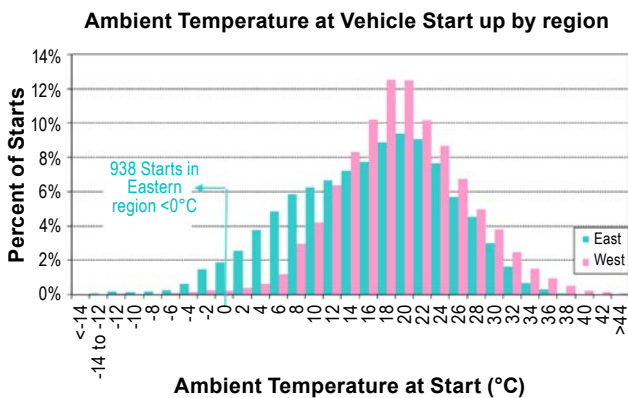
FIGURE 2. 938 Vehicle Starts at Ambient Temperatures <0°C
