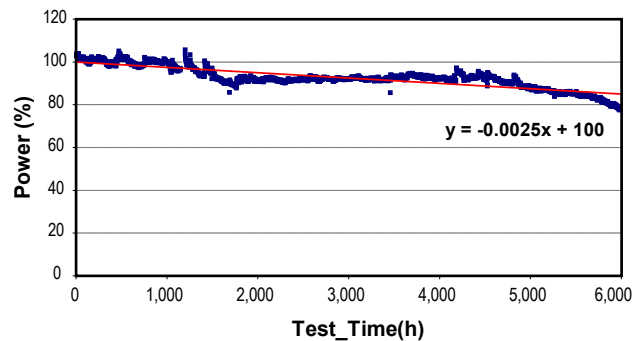
FIGURE 1. Stack/Engine Life Test Demonstrating 6,000 Hours at 5% Decay per 1,000 Hours
