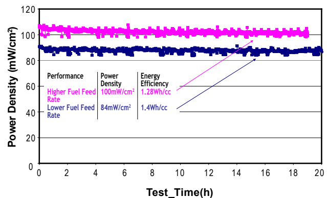
FIGURE 2. MEA Power Density
