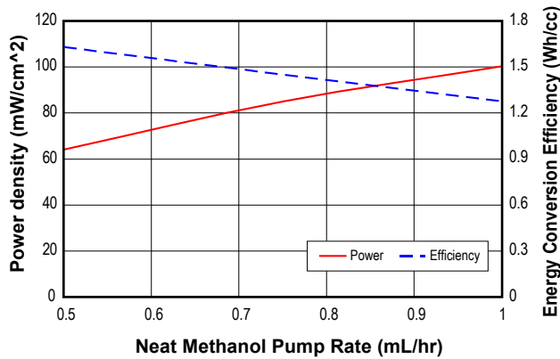
FIGURE 3. Stack/Engine Power Density and Efficiency vs. Pump Rate
