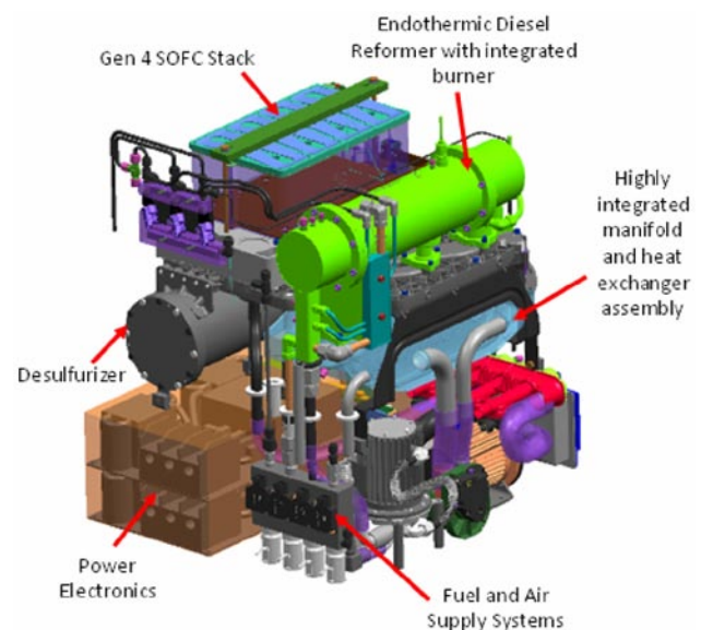
FIGURE 1. DPS3000D Design Level A Layout
