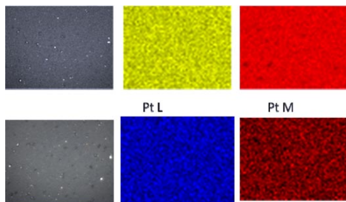
FIGURE 1. Scanning X-ray diffraction of commercial vendor membrane electrode assemblies (MEAs) using two Pt peaks at different energy provides complementary information: L lines show total Pt distribution (both sides of the MEA) and M lines show only one side of MEA.
