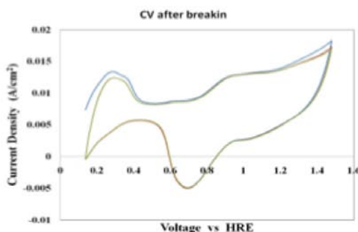
FIGURE 3. Examination of the impact of Diborane (being developed as a hydrogen storage material) as an impurity in the anode feedstream of a 50 cm 2 operating fuel cell. Provided voltage-current curves, alternating current impedance results, and cyclic voltammetry as a function of life testing. Shown is performance after exposure to 40 ppm Diborane for 20 hours.
