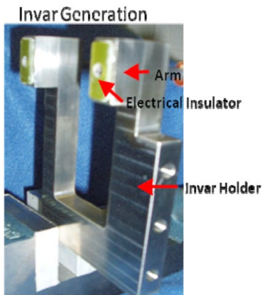
FIGURE 2. LANL designed, built, and provided a new and improved high-resolution fuel cell holder for neutron imaging at the National Institute of Standards and Technology (NIST). The new holder is notable for its uniquely low coefficient of thermal expansion. It has been provided to NIST to make available for all users.
