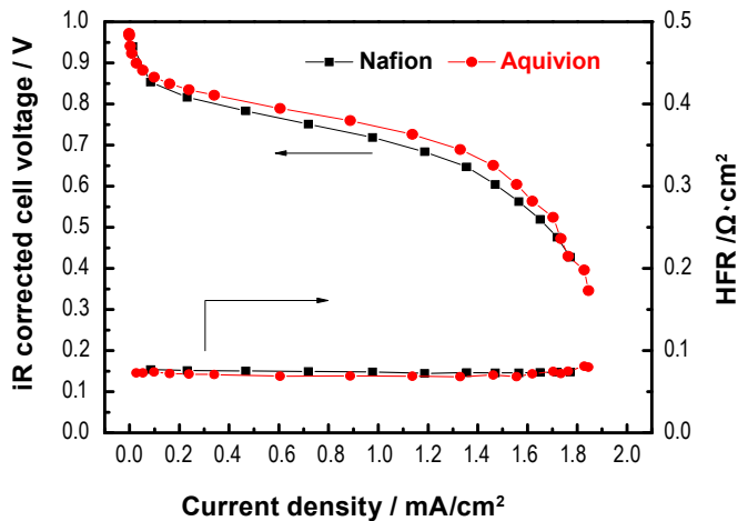
FIGURE 5. Performance comparison of Nafion® and Aquivion®: Evaluation of short-side chain ionomer (Solvay Solexis).
