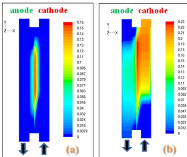
FIGURE 1. Partially two-phase model vs. fully two-phase model – computed liquid saturation contours on the symmetric plane: (a) partially two-phase model; and (b) fully two-phase model.
