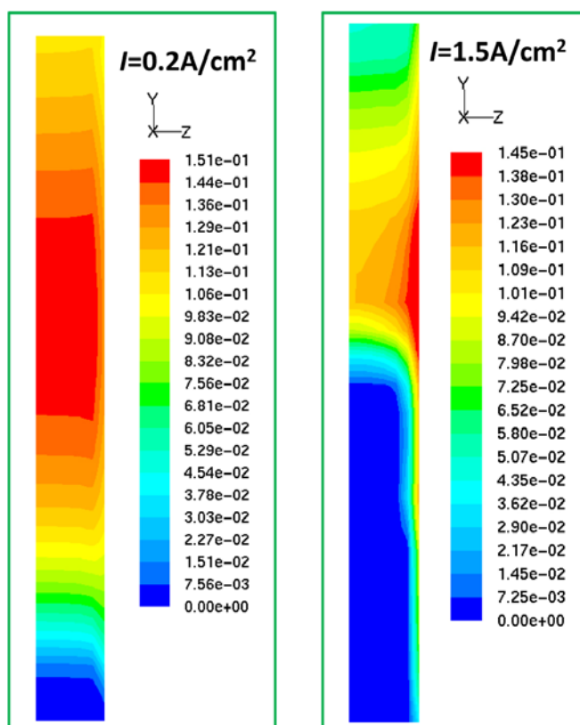
FIGURE 3. Computed liquid-saturation contours at the cathode GFC/GDL interface by the fully two-phase model – effect of current density.
