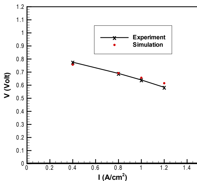
FIGURE 4. Model validation: comparison of measured and computed polarization curves.
