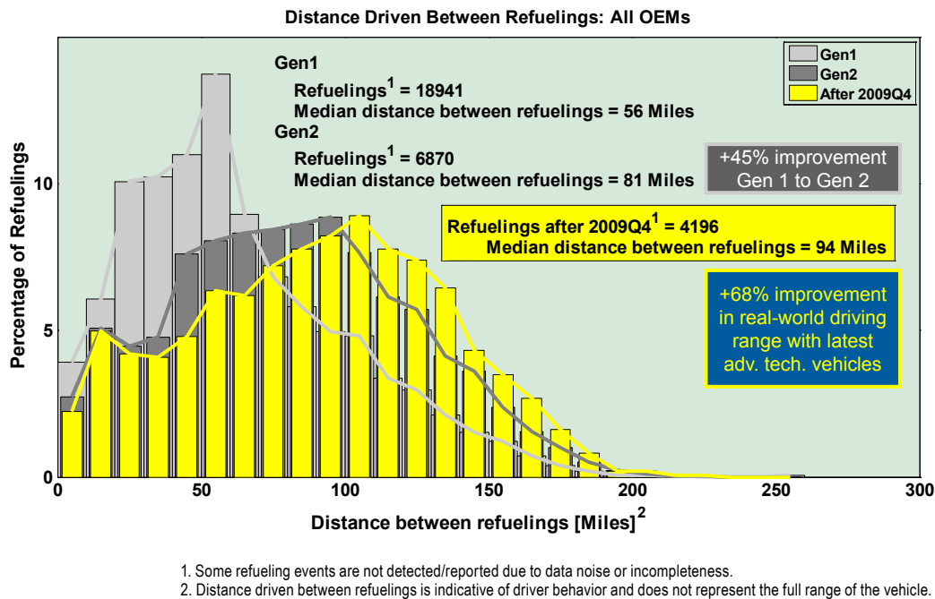
FIGURE 2. Real-World Improvement in Driving Range Between Gen 1, Gen 2, and Latest Advanced Technology Learning Demonstration Vehicles
