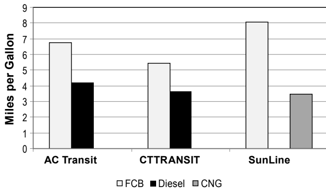
FIGURE 1. Fuel Economy Comparison by Fleet (Diesel Equivalent)
