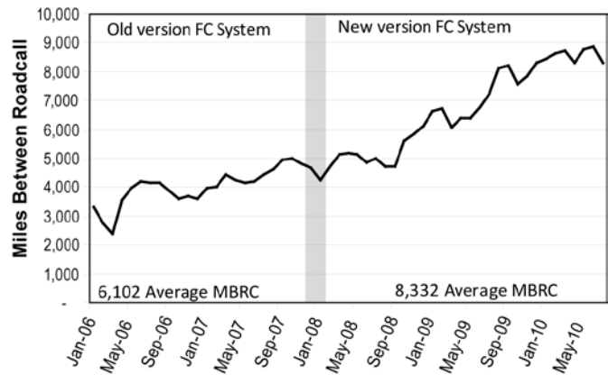
FIGURE 2. Miles between Roadcall for the Fuel Cell Propulsion System (12-Month Rolling Average)
