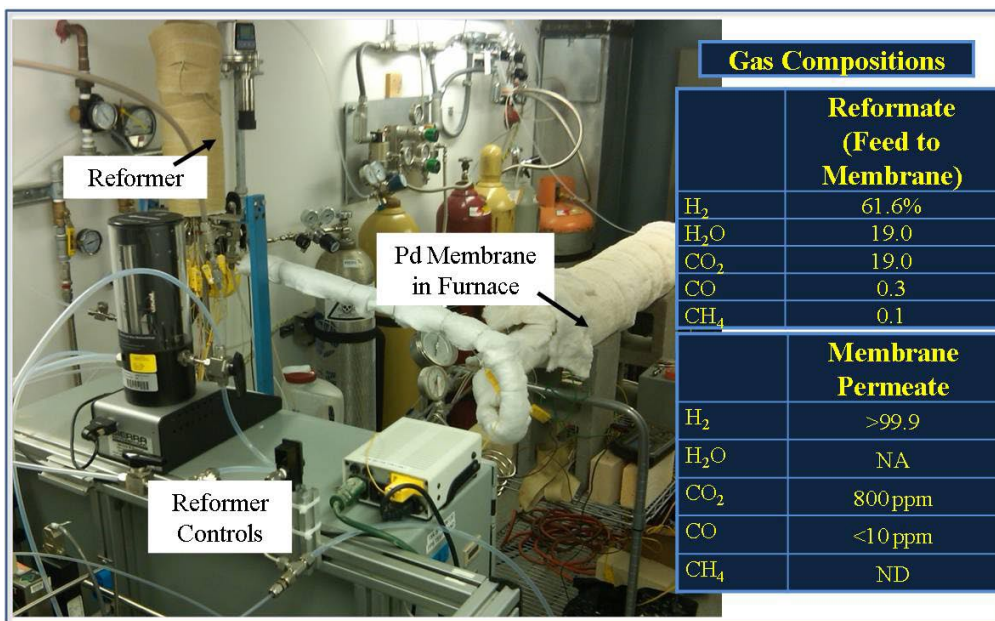
FIGURE 4. Reformer and Hydrogen Selective Membranes Installed and Fully Tested for the Field Test Unit
