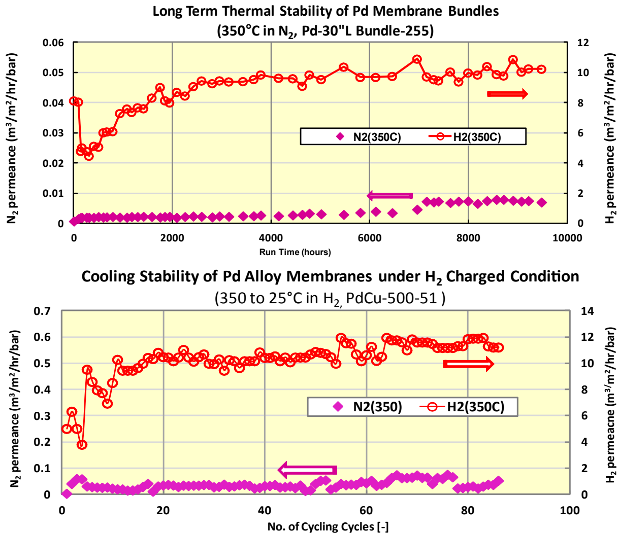
FIGURE 2. Palladium Membrane Stability: Long-Term Thermal Treatment and Cooling under Hydrogen Charged Atmosphere
