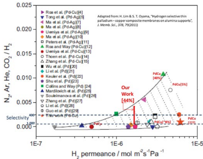
FIGURE 1. Hydrogen Permeances and Selectivity for PdCu Asymmetric Ceramic Membranes: Ours vs. Literature Study
