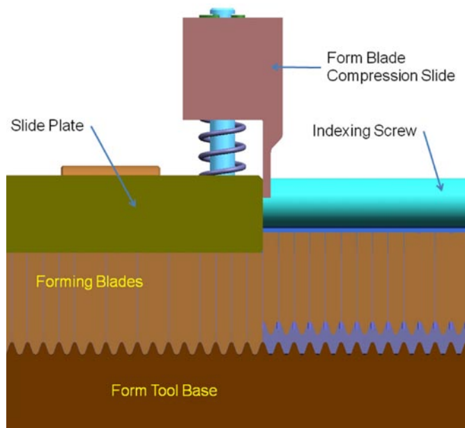
FIGURE 1. Forming Fixture for Corrugating GDL Materials
