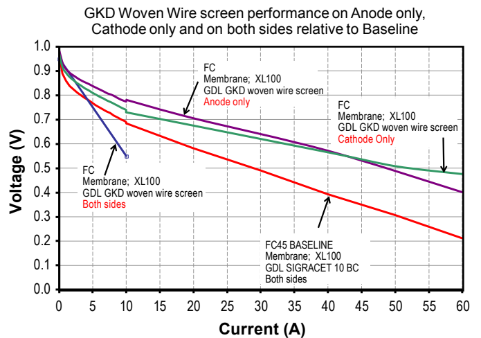
FIGURE 3. GKD Woven Wire Screen Performance
