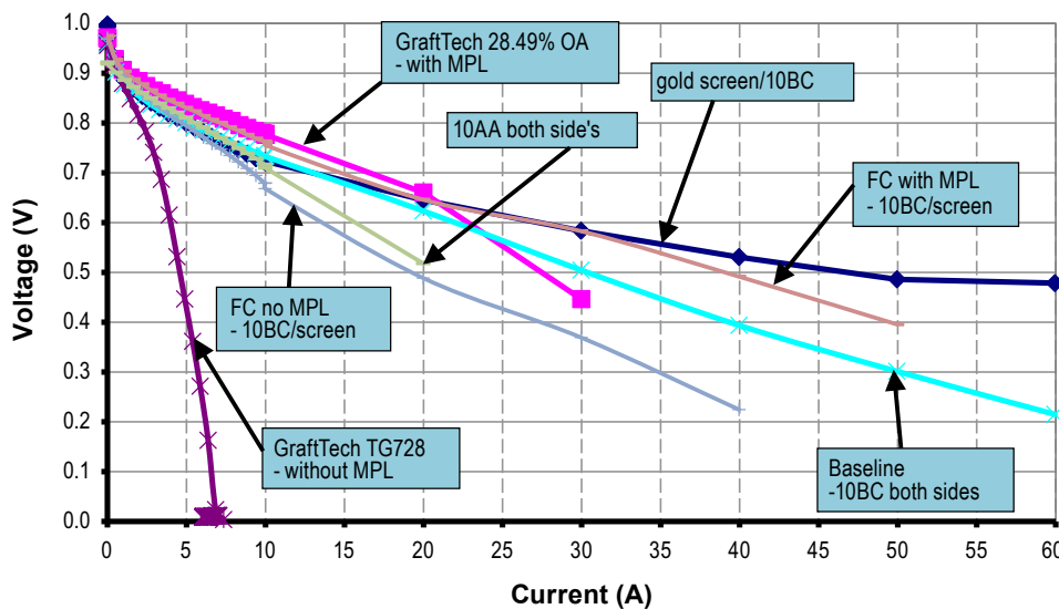
FIGURE 2. Impact of Gas Diffusion Layer Openings/cm 2
