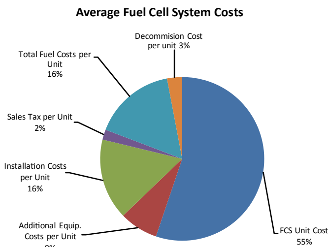
FIGURE 2. Cost Distribution for an Average Micro-CHP FCS in the Deployed Fleet
