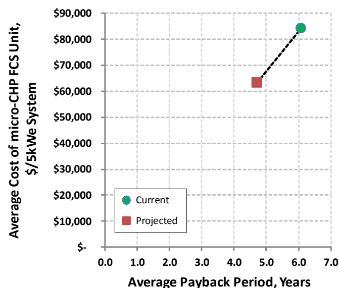
FIGURE 3. Average Payback Period versus Average Cost of the Micro-CHP FCS Unit
