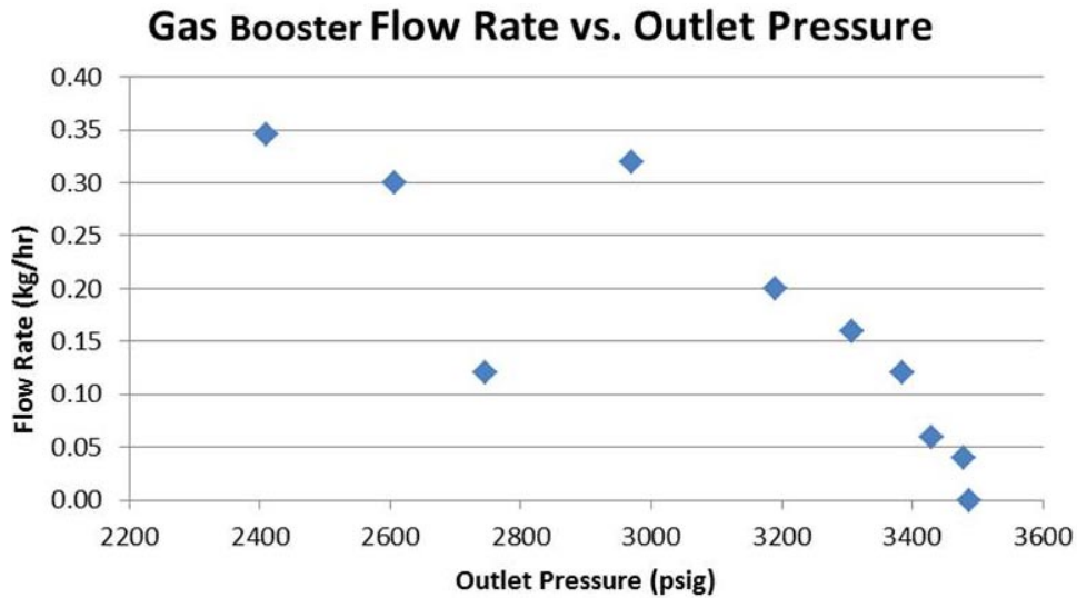
FIGURE 2. Hydrogen Flow Rate versus Gas Booster Outlet Pressure just before Seal Replacement
