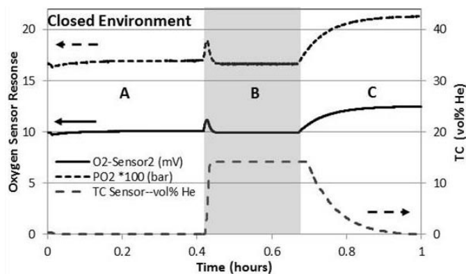
FIGURE 1. Insensitivity of the Oxygen Sensor to a Hydrogen Surrogate in a Closed Environment
