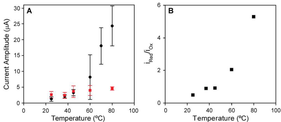
FIGURE 1. Temperature Dependence of (●) H + reduction and (●) hydrogen oxidation catalytic currents and the ratio of the two activities from adsorbed PfSHI . Experiments were performed in a mixed buffer with pH = 6.5 at the indicated temperatures with electrode rotation at 2000 rpm.
