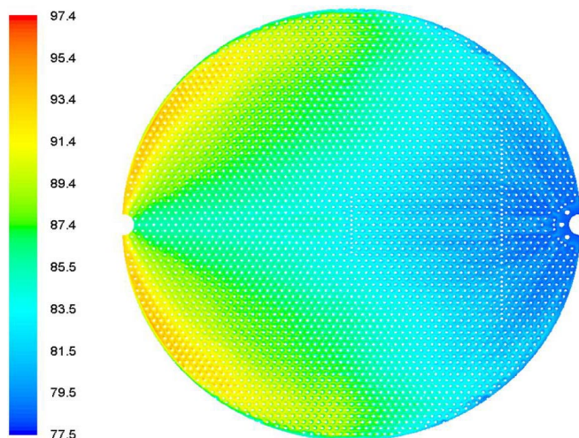
FIGURE 3. Simulation Results for Flow Distribution in a MATI Prototype Cooling Plate
