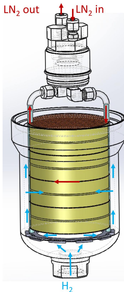
FIGURE 2. 2 Liter Prototype MATI Design
