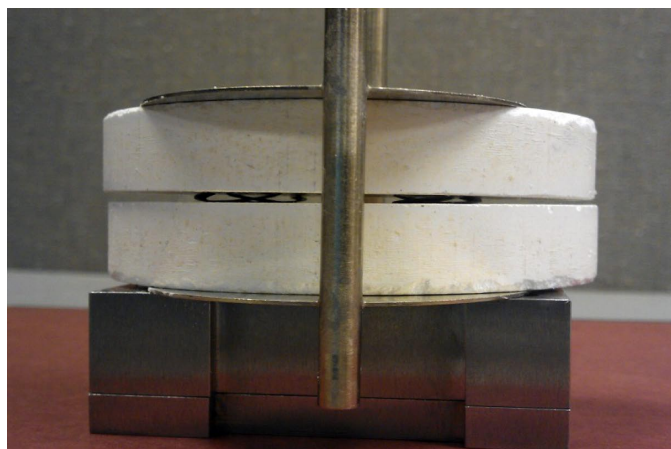
FIGURE 4. Assembled MATI Unit Cell
