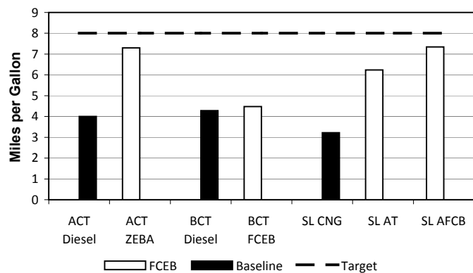
FIGURE 2. Fuel Economy Comparison by Fleet (Diesel Equivalent)
