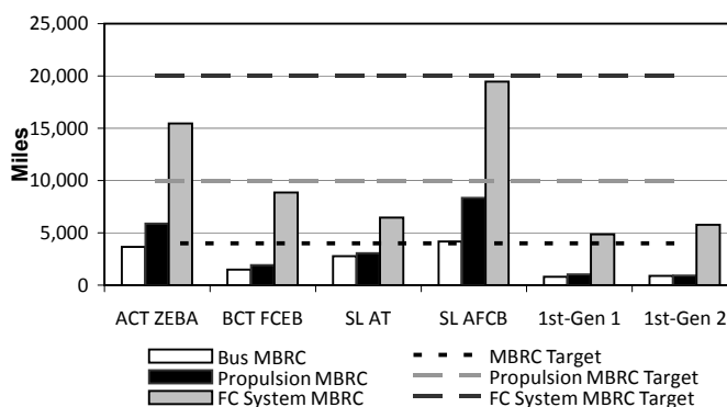
FIGURE 3. Miles Between Roadcall Comparisons by Fleet
