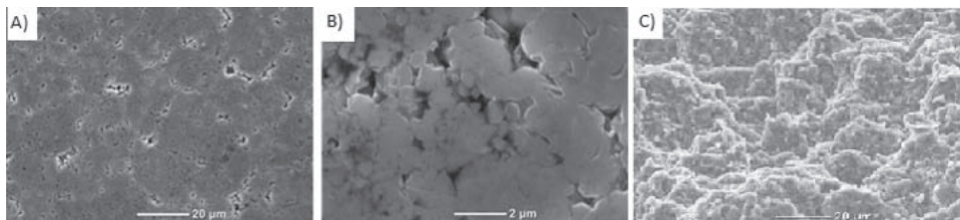
FIGURE 2. (A) SEM image of the surface of a spent alane pellet pressed at 4 tons, (B) increased magnification of the same spent alane pellet, and (C) SEM image of the inside of a broken spent alane pellet
