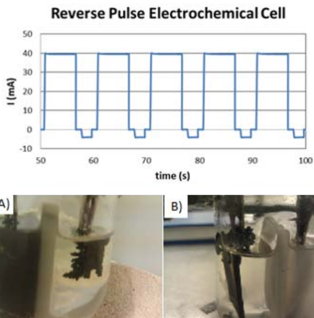
FIGURE 1. Plot of the current vs. time for the reverse pulsing technique used for dendrite formation reduction: (A) anode without reverse pulsing technique and (B) anode with reverse pulsing technique
