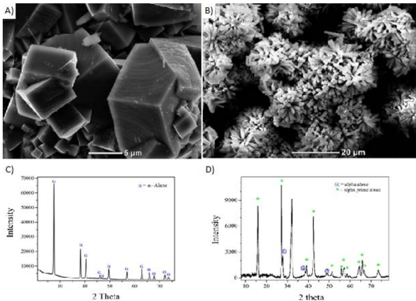
FIGURE 3. (A) SEM image of alpha-alane crystals, (B) SEM image of alpha prime crystals, (C) XRD pattern of pure alpha alane, and (D) XRD pattern of alpha prime alane with trace alpha alane
