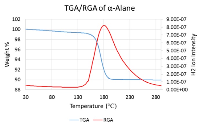
FIGURE 4. TGA/RGA of \alpha -alane displaying >9 wt% H 2
